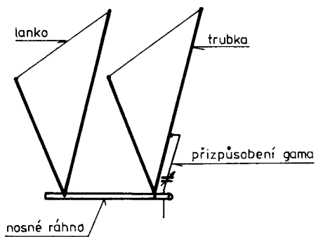
Obr.58. Anténa "delta loop"
